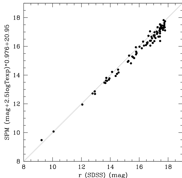
Fig. 5. Comparison between the integrated r mag from SDSS (DR10, except for the 10 brightest objects, measured as in Section 2.3) and the magnitudes measured in the r images taken at SPM in 2014, using the IRAF task QPHOT.
