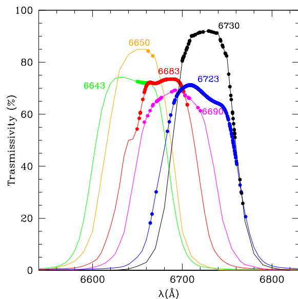
Fig. 3. The transmissivity of the ON-band (6643, 6650, 6683, 6690, 6723 and 6730 Å) filters. Points mark the throughput at the redshift of the target galaxies..
