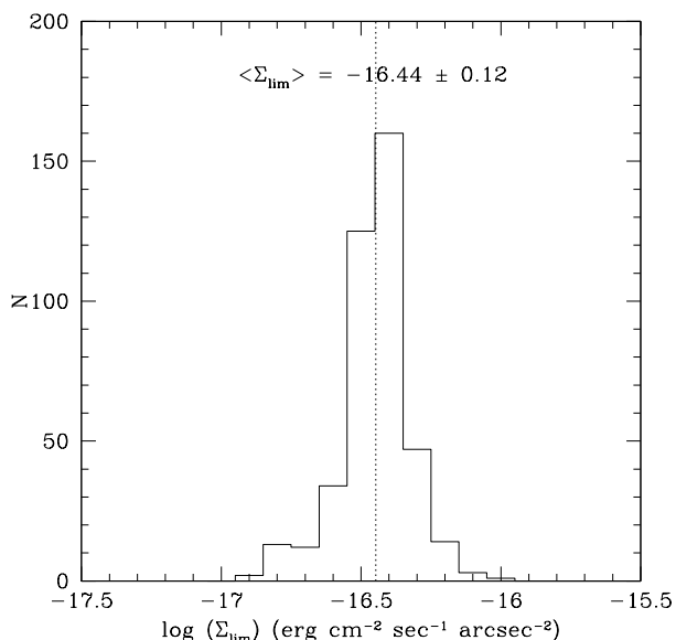
Fig. 8. Histogram of the limiting 1\sigma surface brightness in the H \alpha NET images.
