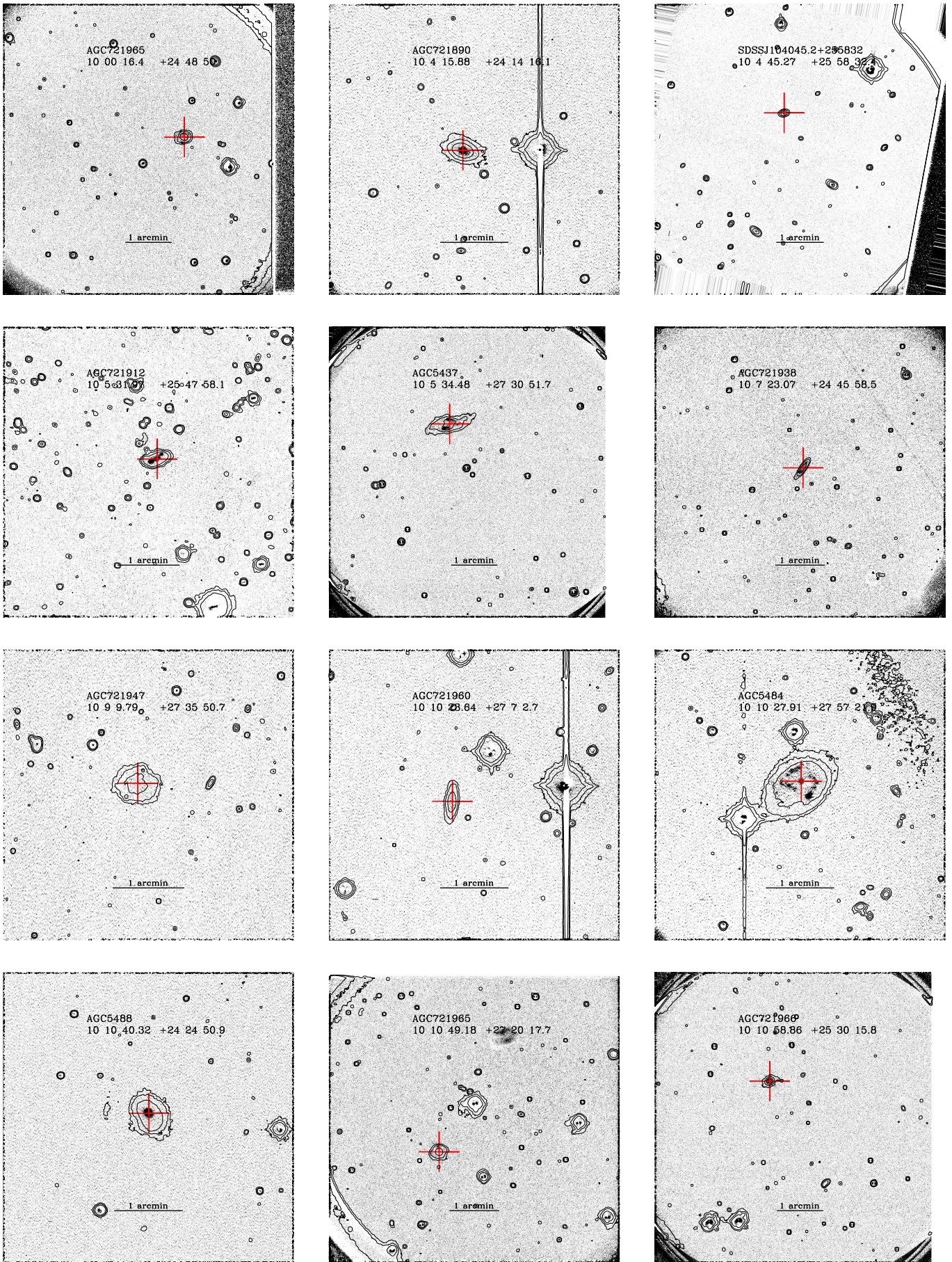
Fig. A.1. One page gallery of the atlas of 724 galaxies (red crosses) observed in H\alpha , identified by their celestial coordinates and, if available, by their AGC designation. The OFF-band contours are drawn at 1.5, 2.5, 5\times\sigma of the sky in the normalized r band images. The grey scale represents the NET flux intensity between 1 and 3\times\sigma of the sky in the H\alpha NET (continuum subtracted) frames. A 1 arcmin bar is given on all images. All 2013 images have been rotated by 10.5 or 3.5 clockwise to align the Y axes of the CCD with the North direction.
