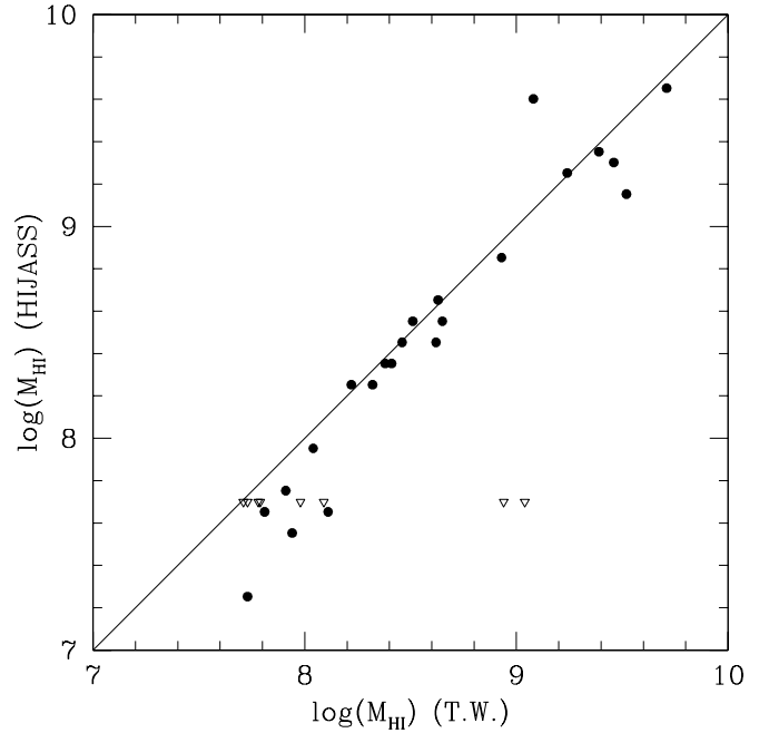
Fig. 4. Comparison of the HI masses as derived from this work with those derived in the blind HIJASS HI survey (Davies et al. 2004) for galaxies in common in the radial velocity interval of 500\text{--}2500\text{ km s}^{-1} . Open triangles are for undetected HIJASS galaxies.
