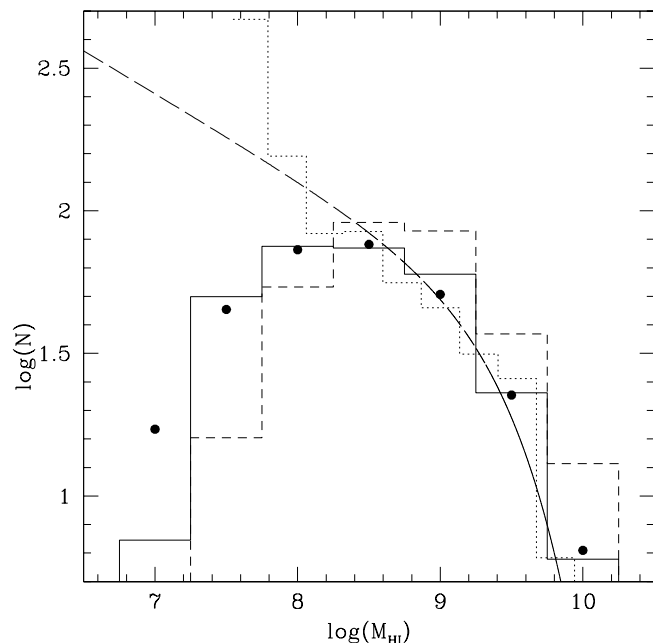
Fig. 6. The dotted histogram is obtained from the late-type galaxies optical luminosity function, as determined in the field by Marzke et al. (1998), transformed into M_{HI} using the relation \log M_{HI} = 2.9 - 0.34 \times M_p discussed in the text. It appears consistent with the field HILF of Zwaan et al. (2003) (long dashed line) indicating that most of the H I is contributed to by late-type galaxies. The dashed histogram is obtained from the late-type galaxies optical luminosity function of Virgo (see Fig 7), transformed into M_{HI} using the same M_{HI} vs. M_p relation. The continuum histogram is the HIMF actually observed in Virgo (see Fig. 5). The filled dots represent the Monte Carlo simulation described in the text aimed at modeling the effects of the H I deficiency on the HIMF.
