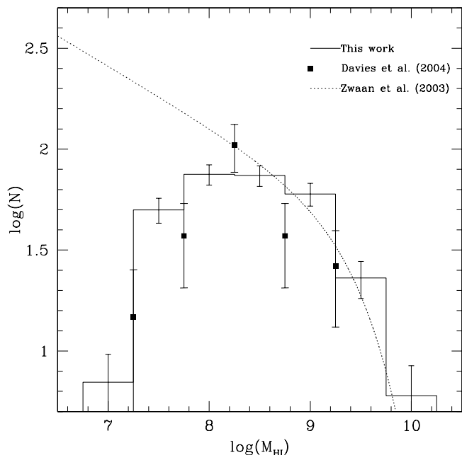
Fig. 5. The Virgo cluster H I mass function (HIMF) as derived from this work using only the detected galaxies (histogram), together with the HIMF derived from the blind HIJASS survey (D04), normalized to our data as described in the text. Error bars represent purely statistical errors. For comparison, the dotted line gives the Field HIMF as derived by Zwaan et al. (2003), normalized arbitrarily in order to match our data at M_{HI} = 10^{9.5} M_{\odot} .
