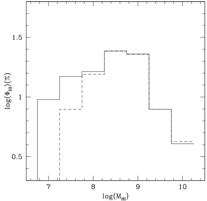
Fig. 8. The fractional HI mass function as derived from the detected objects alone (dashed histogram) and including undetected galaxies (continuum histogram).
