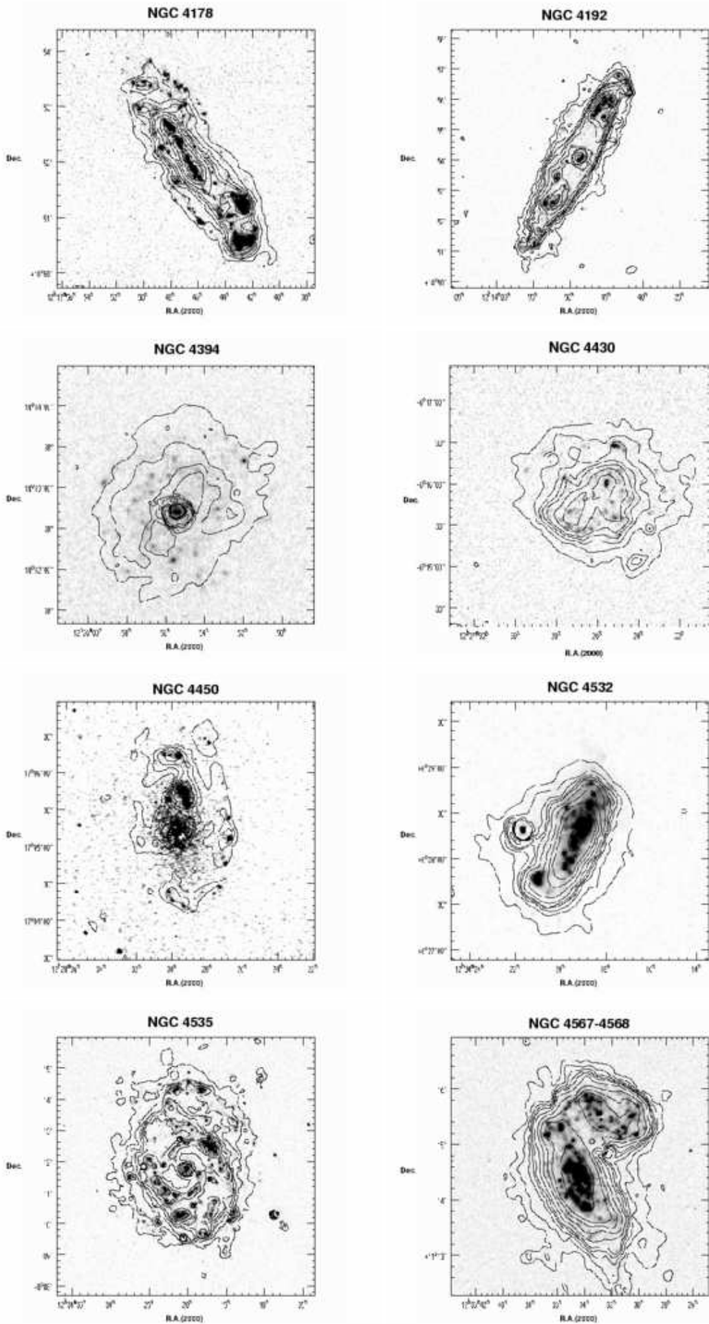
Fig. 5. The contour plot of the 6.75 \mu\text{m} dust emission (without the contribution of the stellar emission) superimposed on the gray
